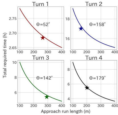
Fig. 13 Estimated total required time ( T ) and its dependency on approach run length ( L ). Actual time–length point for each turn is indicated by a star.
